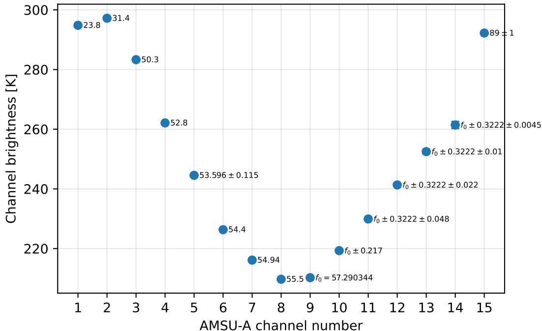
AMSU-A-like channelized measurements
