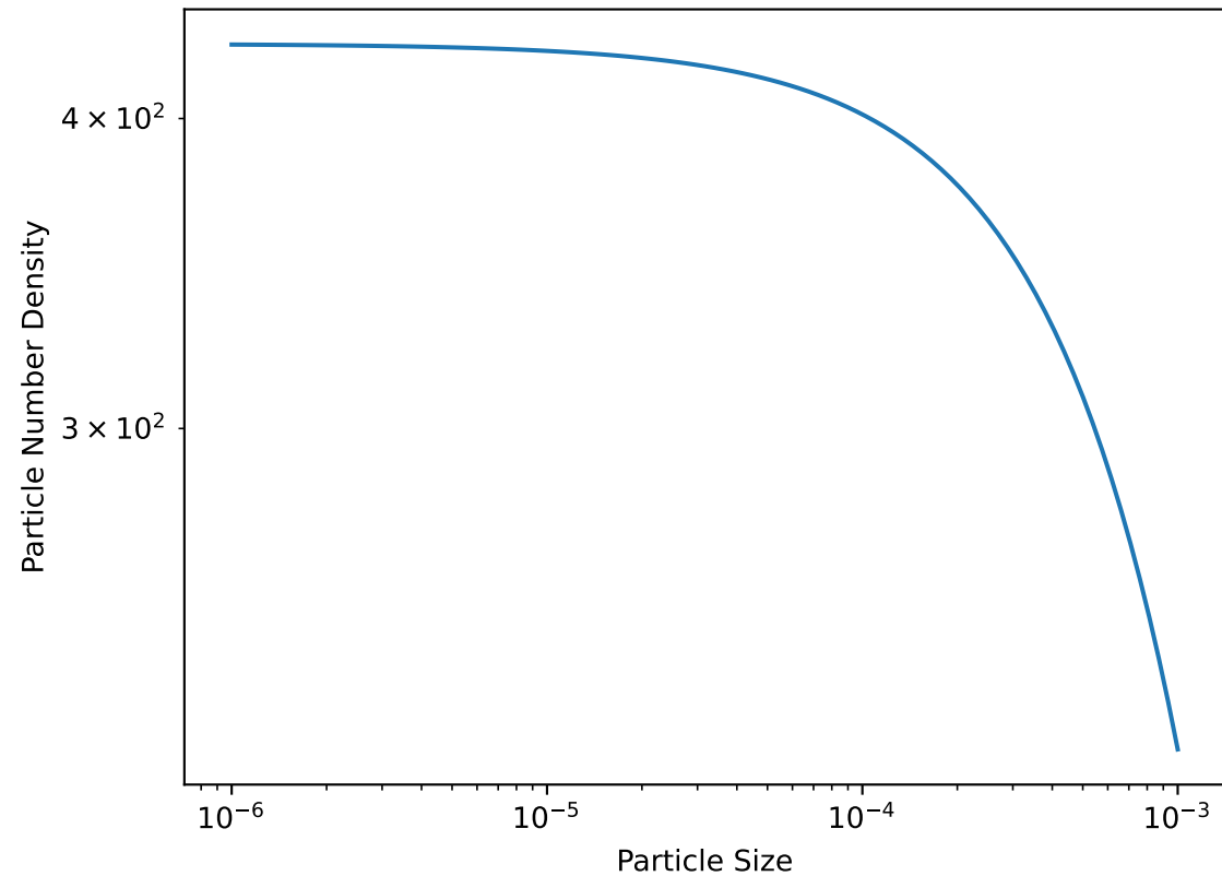
Single-moment modified gamma distribution
