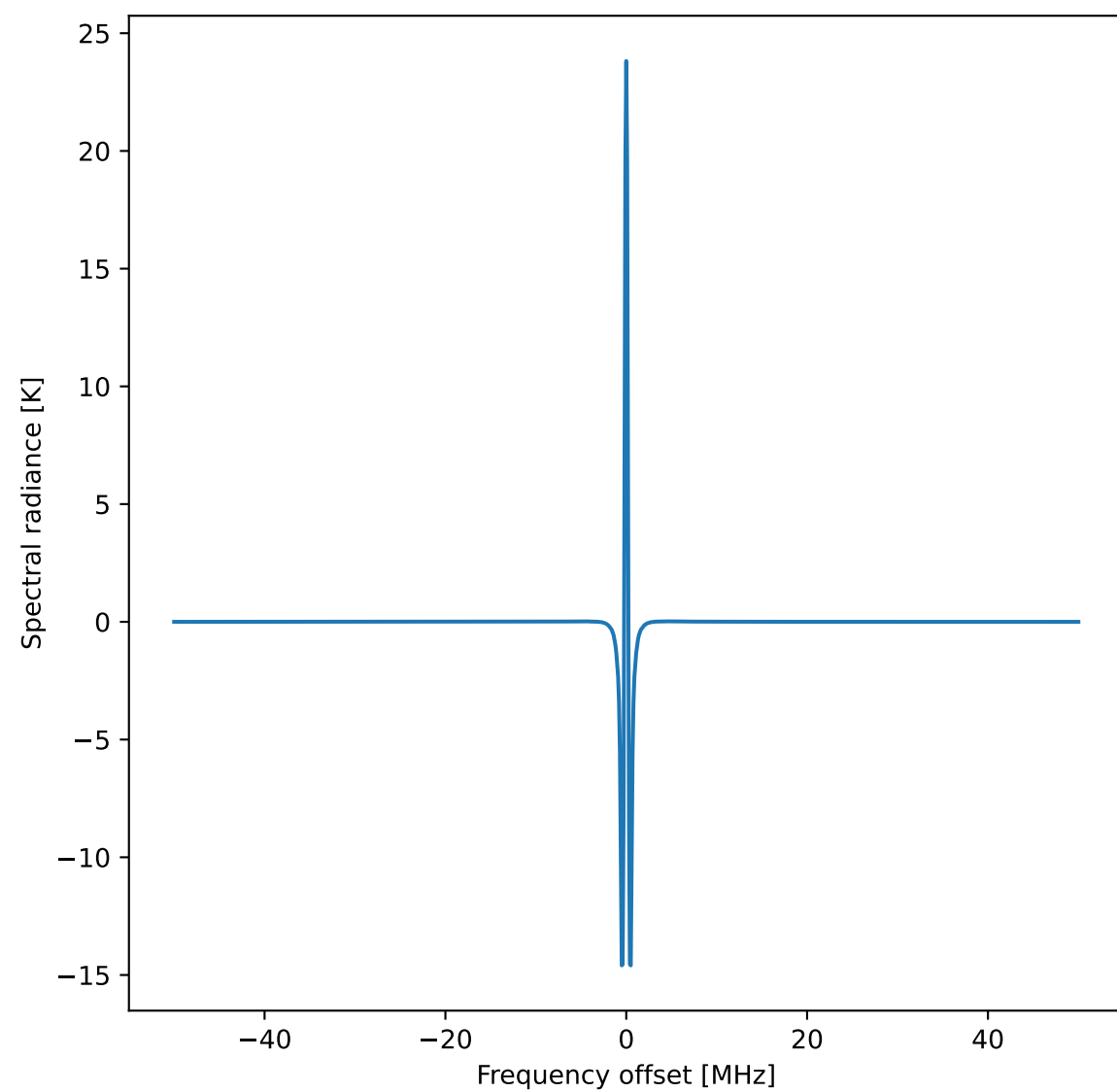
Zeeman effect of 118750 MHz O 2 line
