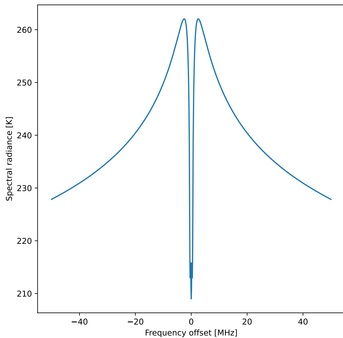
Zeeman effect of 118750 MHz O 2 line
