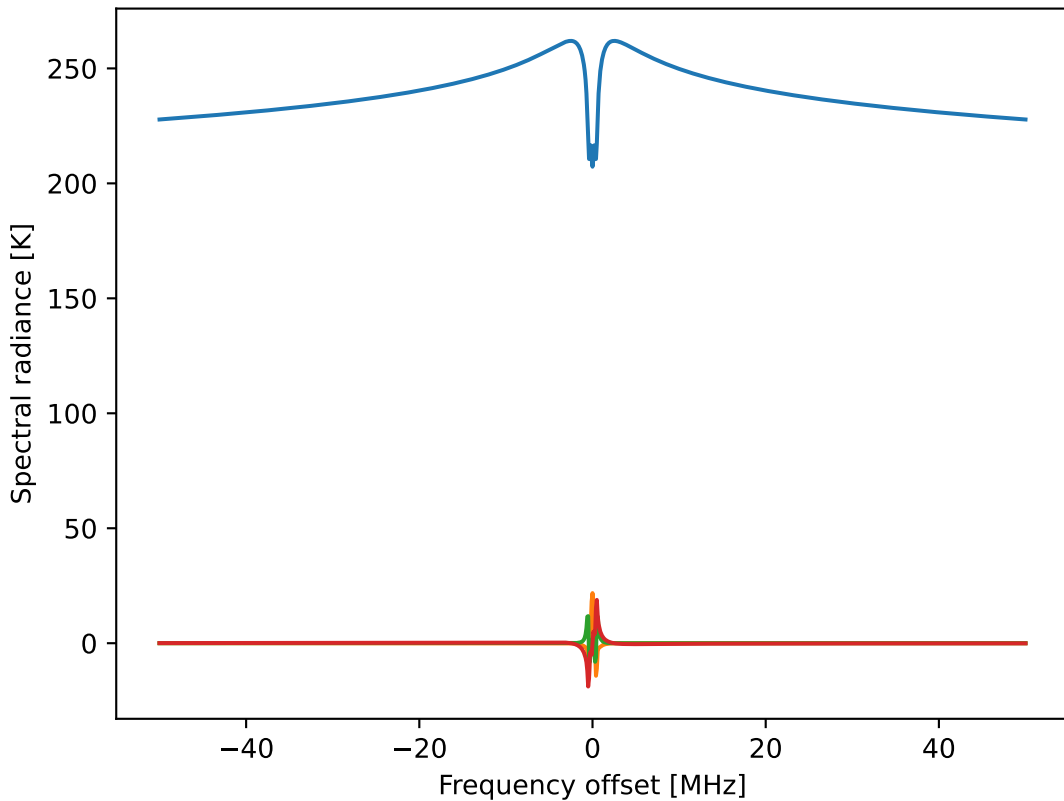
Zeeman effect of 118750 MHz O 2 line
