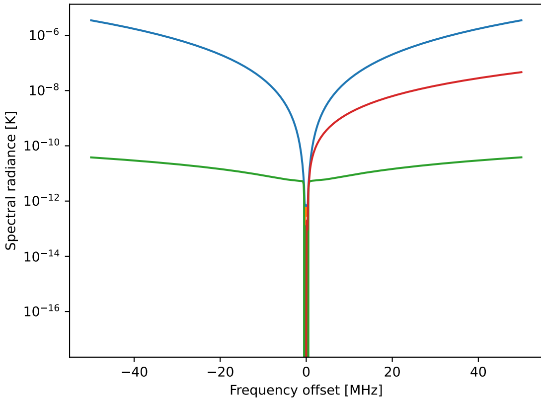
Zeeman effect of 118750 MHz O 2 line
