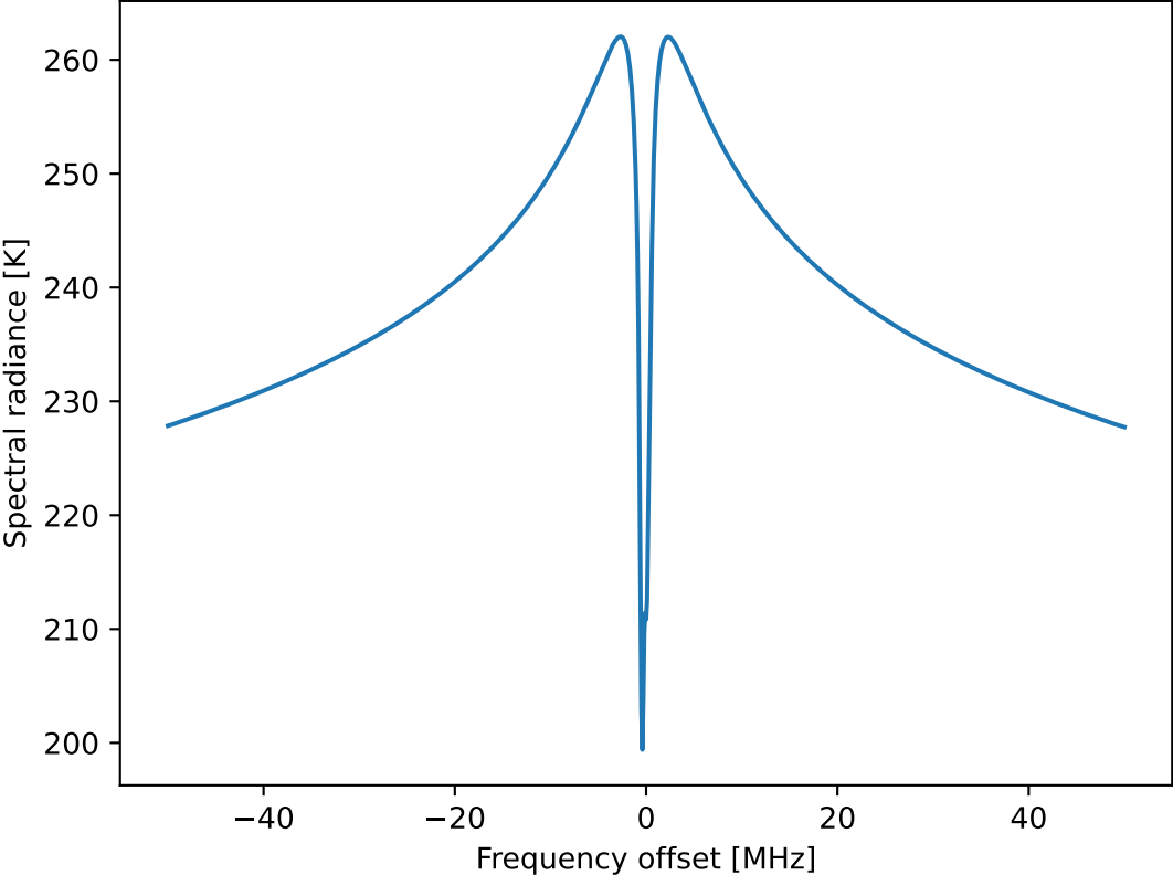
Zeeman effect of 118750 MHz O 2 line with Gaussian channels on individual grids
