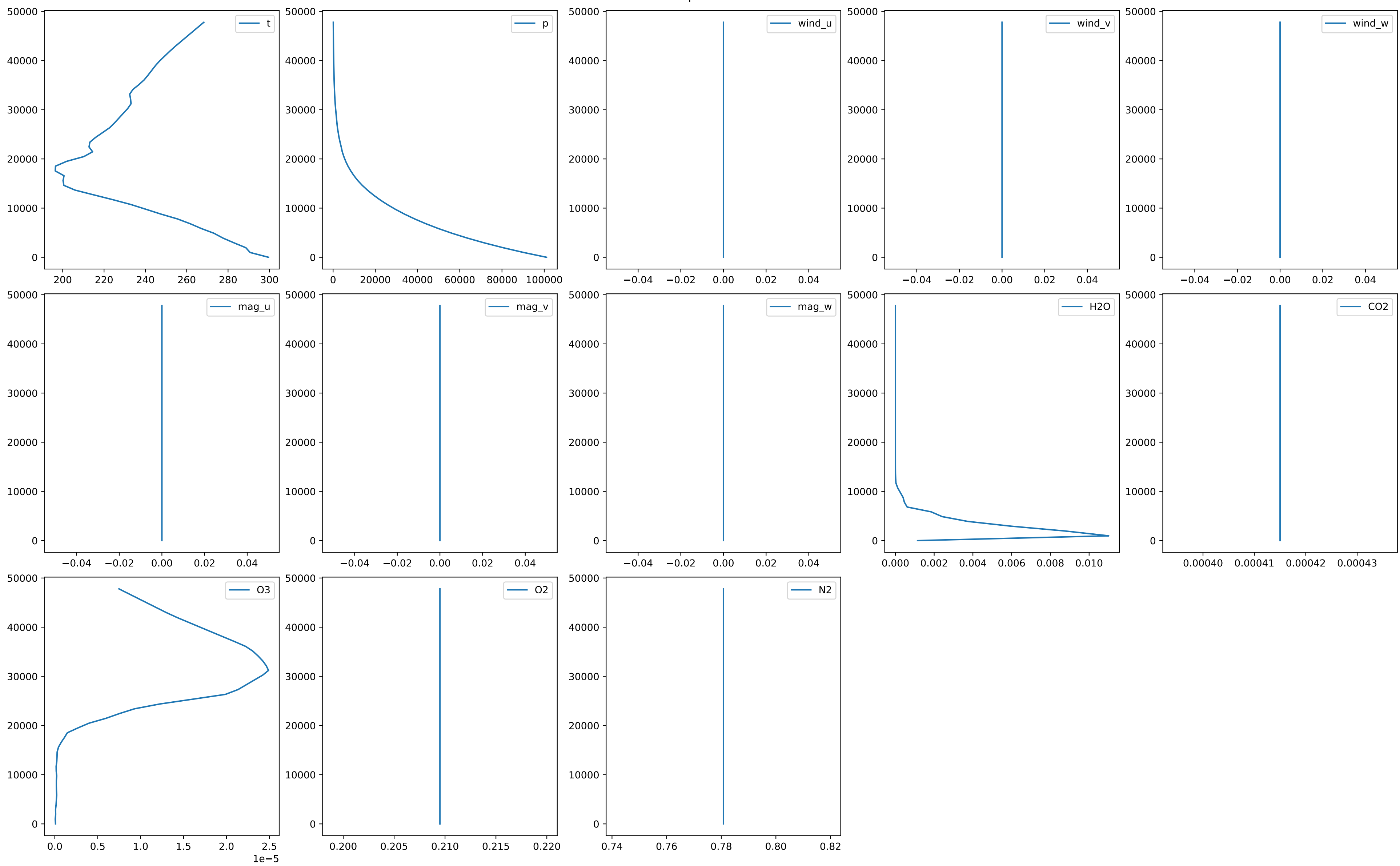
Atmospheric field
