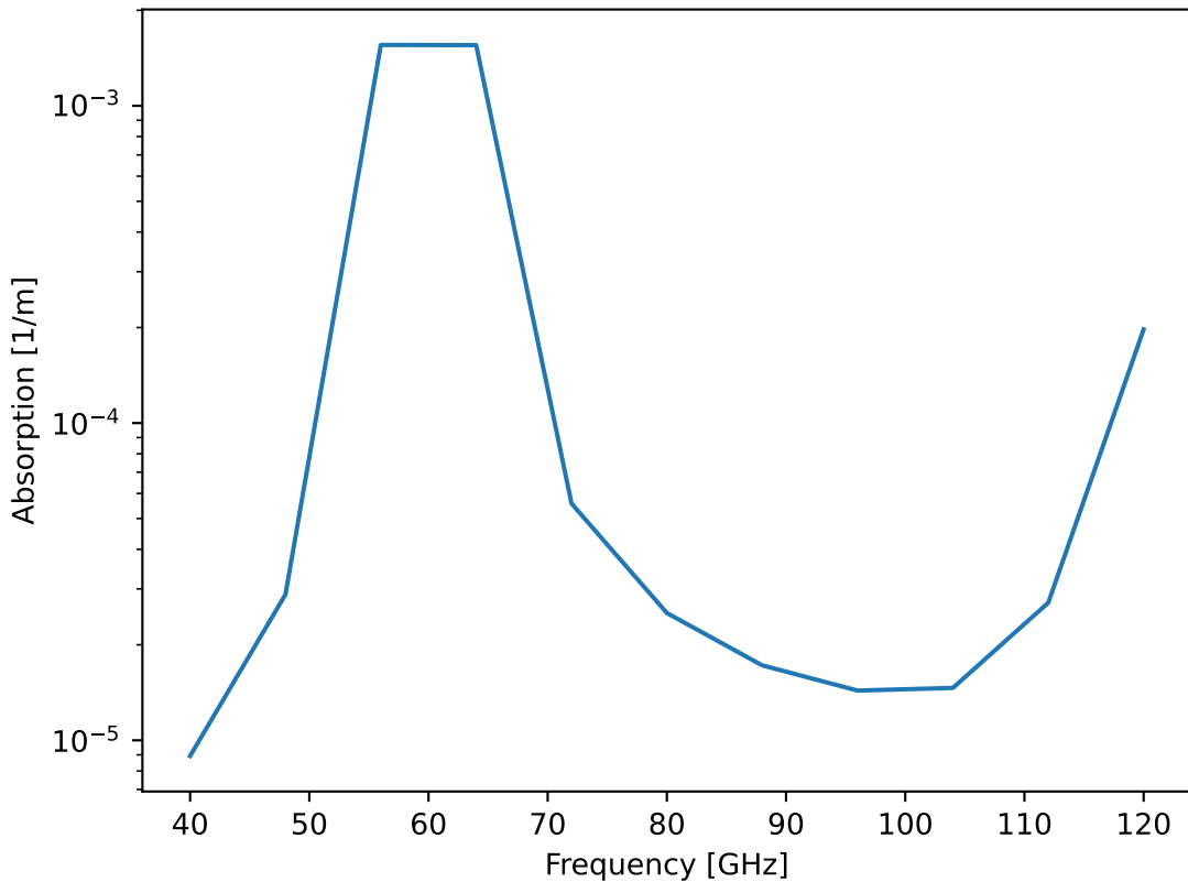
O2-66 absorption from examples/arts-cat-data/lines/lines.py
