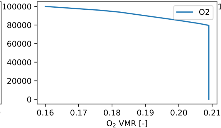
O 2 VMR profile
