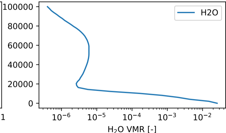
H 2 O VMR profile
